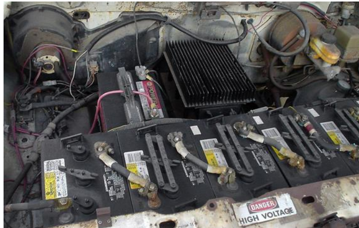
Gambar 10.23 1993 Ford Ranger “kotak ajaib.”
