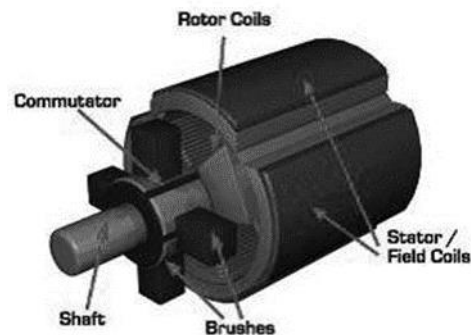
Gambar 6.6 Motor DC dengan stator bulat (Courtesy of Zero Emission Vehicles of Australia dan www.electric-cars-are-for-girls.com ).
