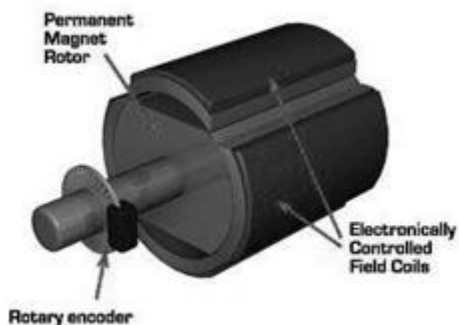
Gambar 6.5 Motor DC Brushless (Courtesy of Zero Emission Vehicles of Australia dan www.electric-cars-are-for-girls.com ).
