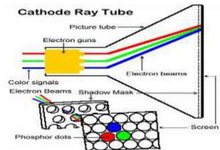
Gambar 3.11 CRT
