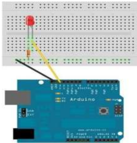
Gambar 16. Rangkaian Blinking LED
