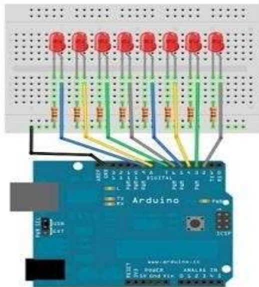
Gambar 17. Skema Running Led
