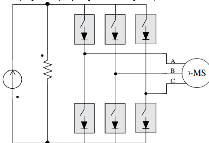
Gambar 9.14 Inverter sumber arus.
