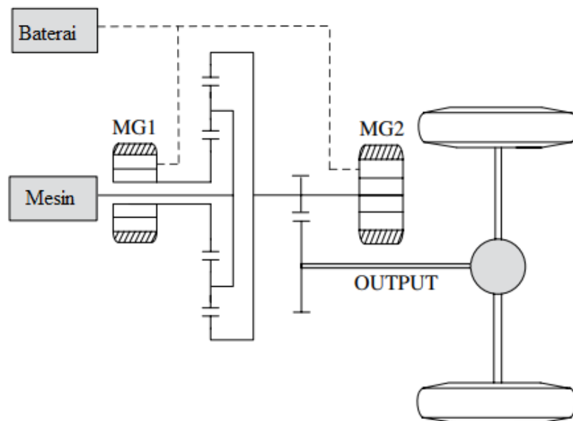
Gambar 4.3 Transmisi Toyota Prius
