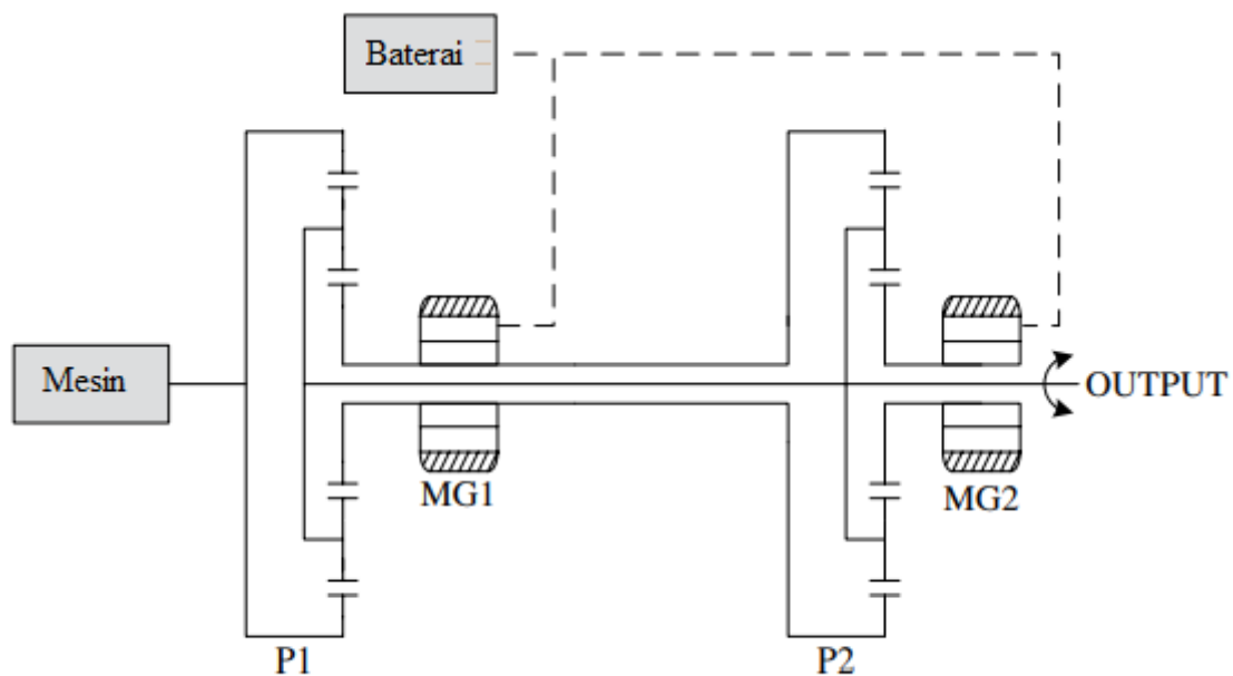
Gambar 4.7 High Range
