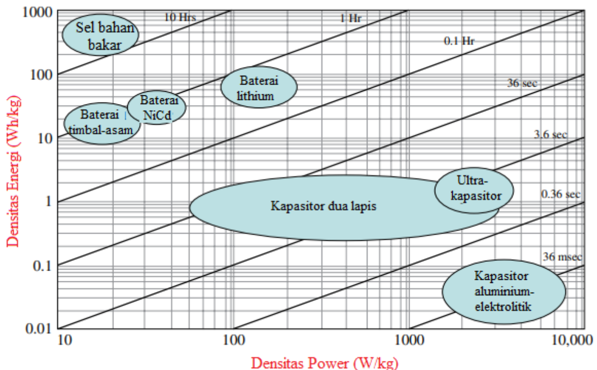
Gambar 11.15 Perbandingan densitas daya ESS dan densitas energi dalam HEV. Sumber: Courtesy of the U.S. Department of Defense
