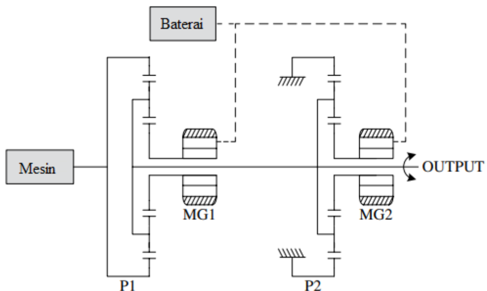
Gambar 4.6 Low Range.
