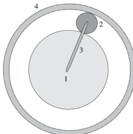
Gambar 4.1 Roda gigi planet: 1, sun gear; 2, planetary gear; 3, planetary arm atau carrier; 4, ring gear.
