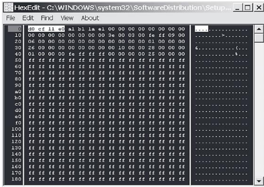
Gambar 4.16 Tanda Tangan File Dokumen MS Word Office 2003
